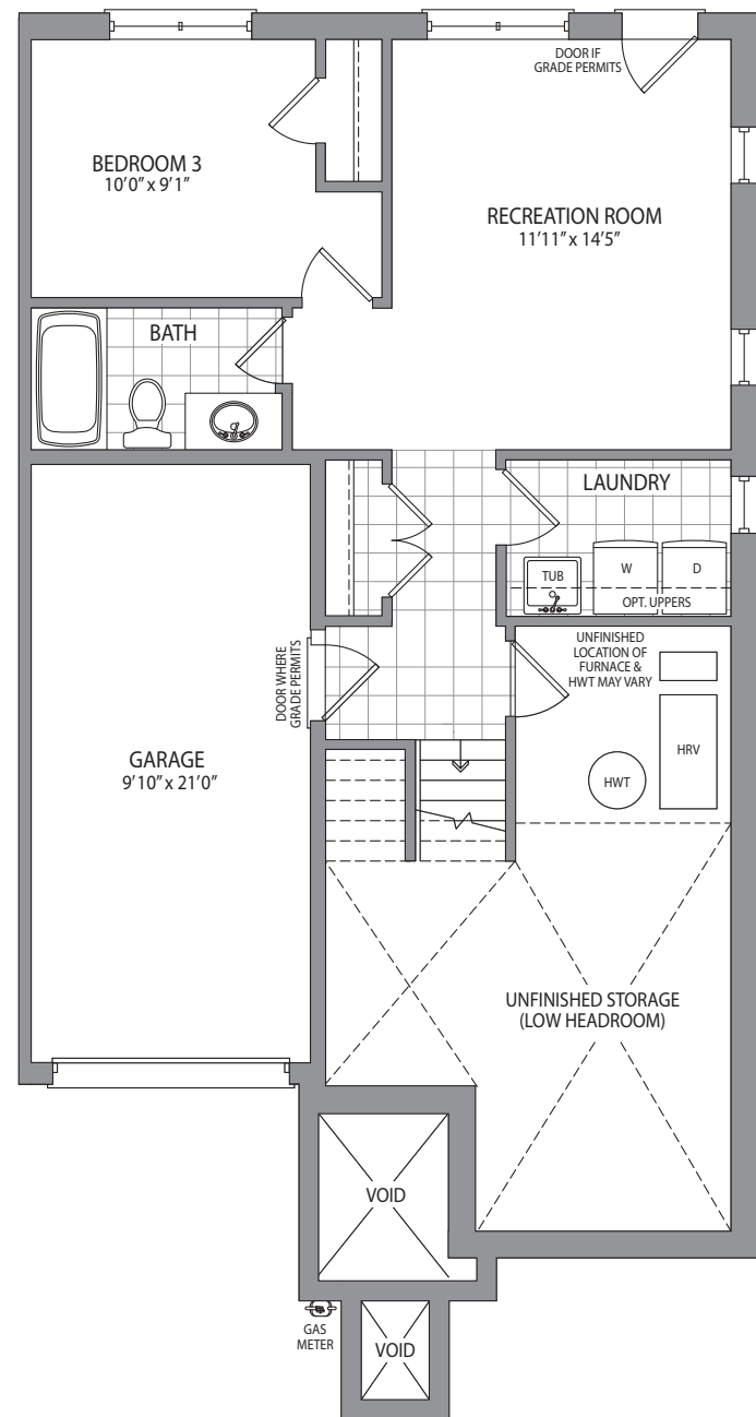
OPT. 3 BEDROOM LOWER LEVEL A1
