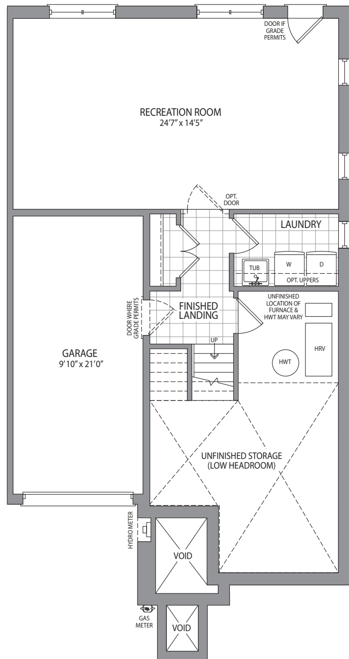
LOWER LEVEL A1
