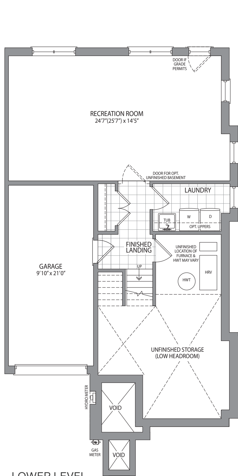
LOWER LEVEL EXTERIOR END A2
